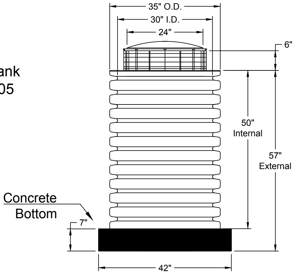
Side View
